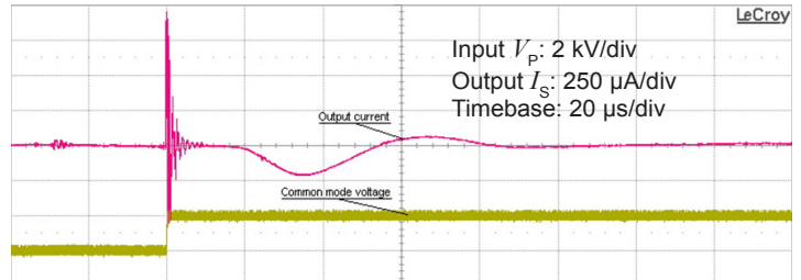
Figure 12: Detail of typical common mode perturbation (2000 V step with 6 kV/μs, R_M = 100 \Omega )
