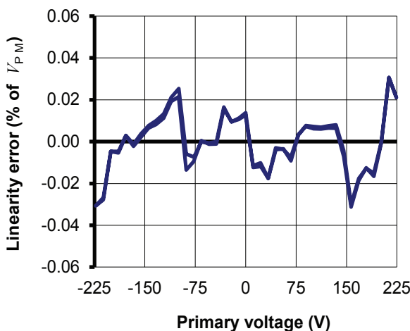
Figure 15: Typical linearity error at 25 °C
