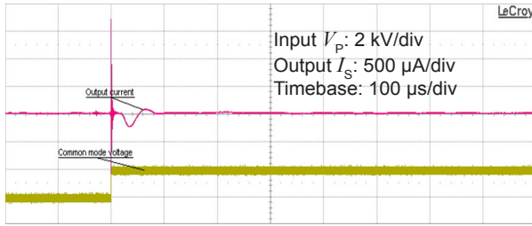
Figure 11: Typical common mode perturbation (2000 V step with 6 kV/μs R_M = 100 \Omega )
