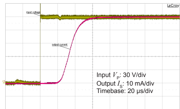
Figure 6: Typical step response (0 to 150 V)
